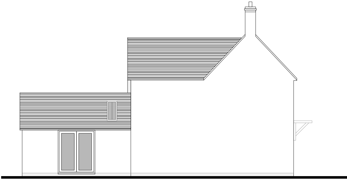
Existing Side Elevation at 1:100 scale NORTH EAST
