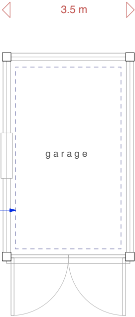
Proposed Plan at 1:100 scale
