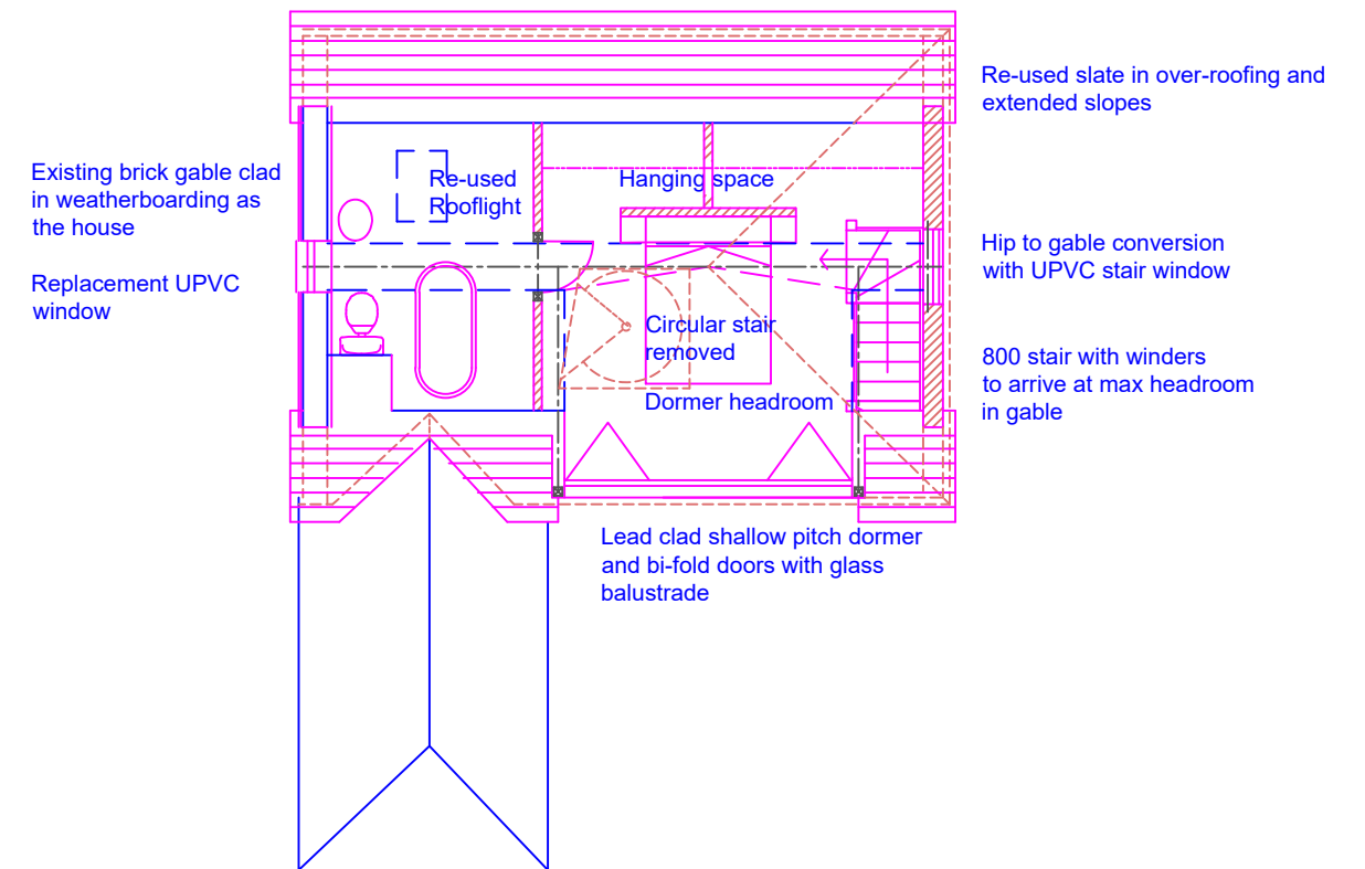
FIRST FLOOR
