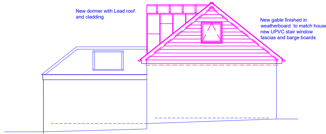
NORTH ELEVATION
