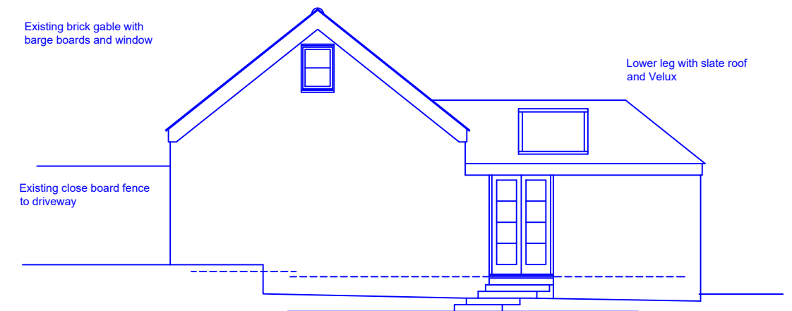
SOUTH ELEVATION
