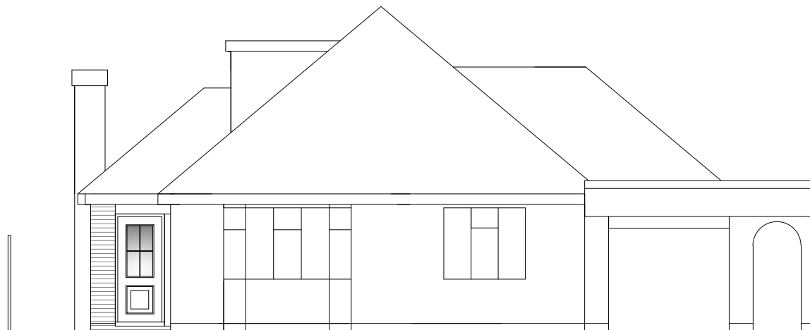
FRONT ELEVATION (EAST)
