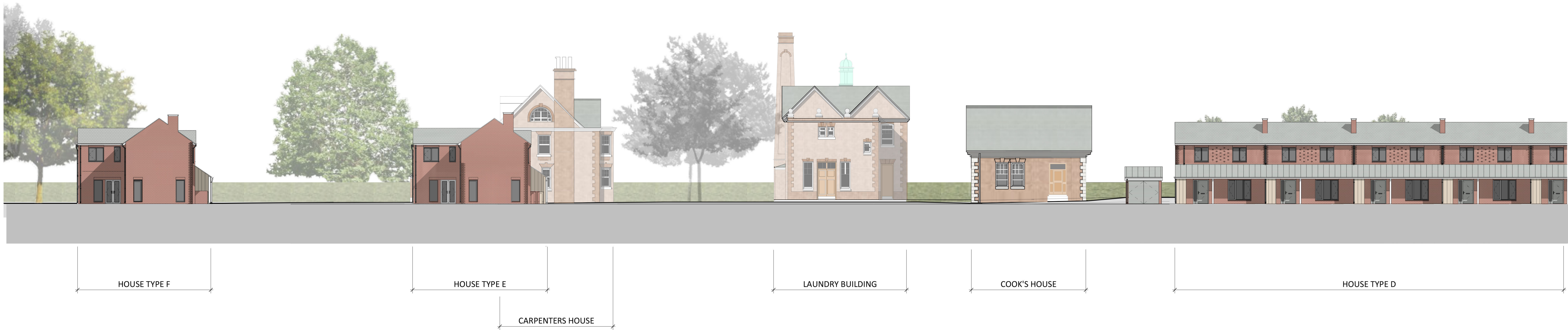
PROPOSED WEST STREET ELEVATION BB Scale: 1 : 200
