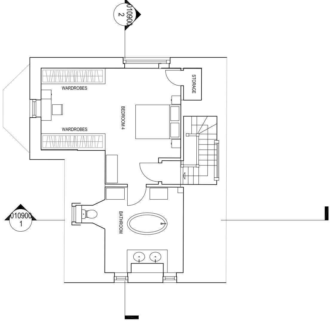
Second Floor Plan Scale: 1 : 100
