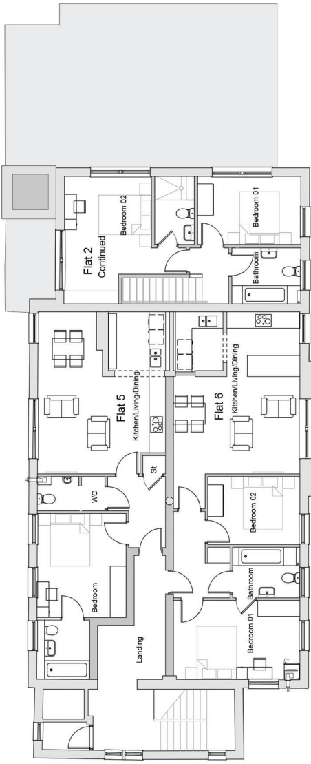
2 First Floor Plan Scale: 1:100
