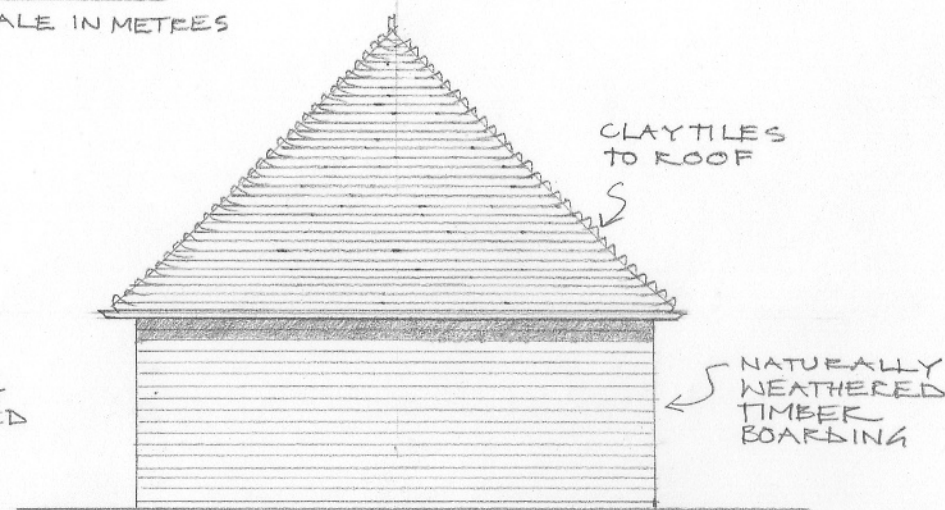
REAR ELEVATION PLOT 1 & 2
