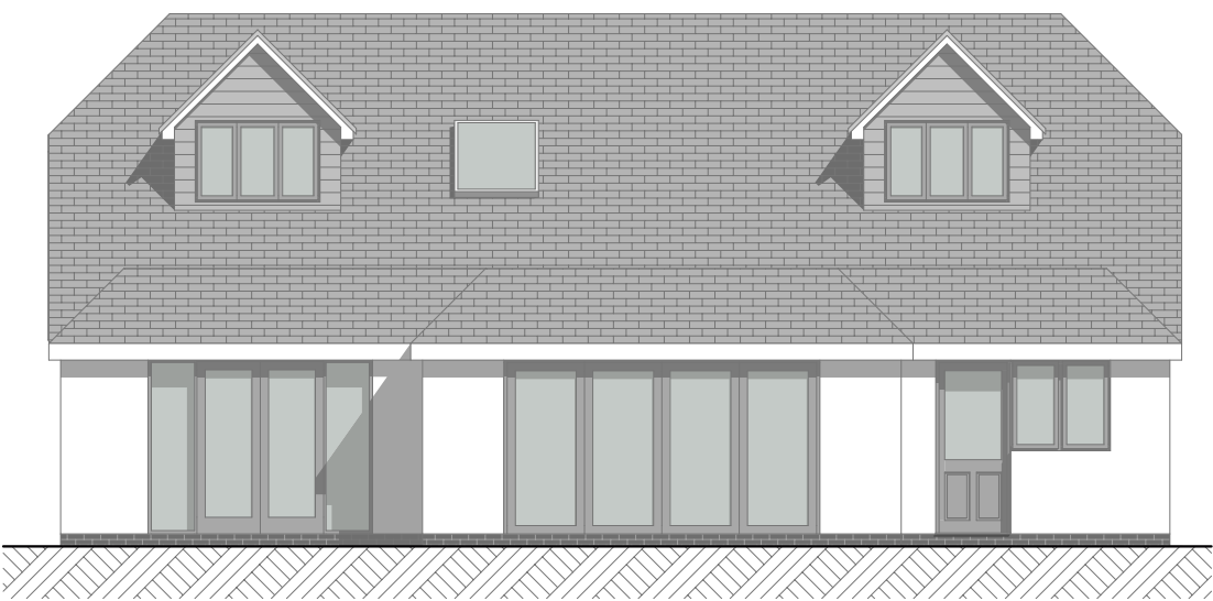
NORTH ELEVATION
