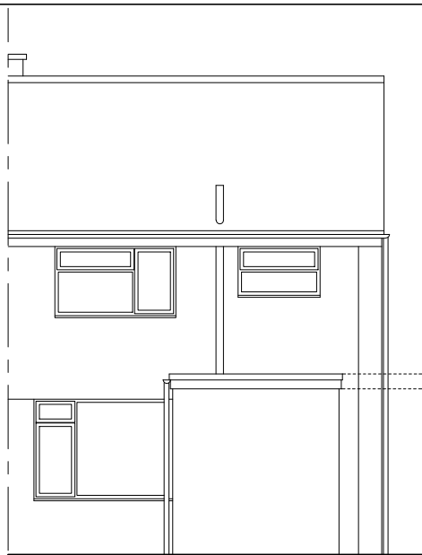
Existing West Elevation (rear) 1:100 @ A3
