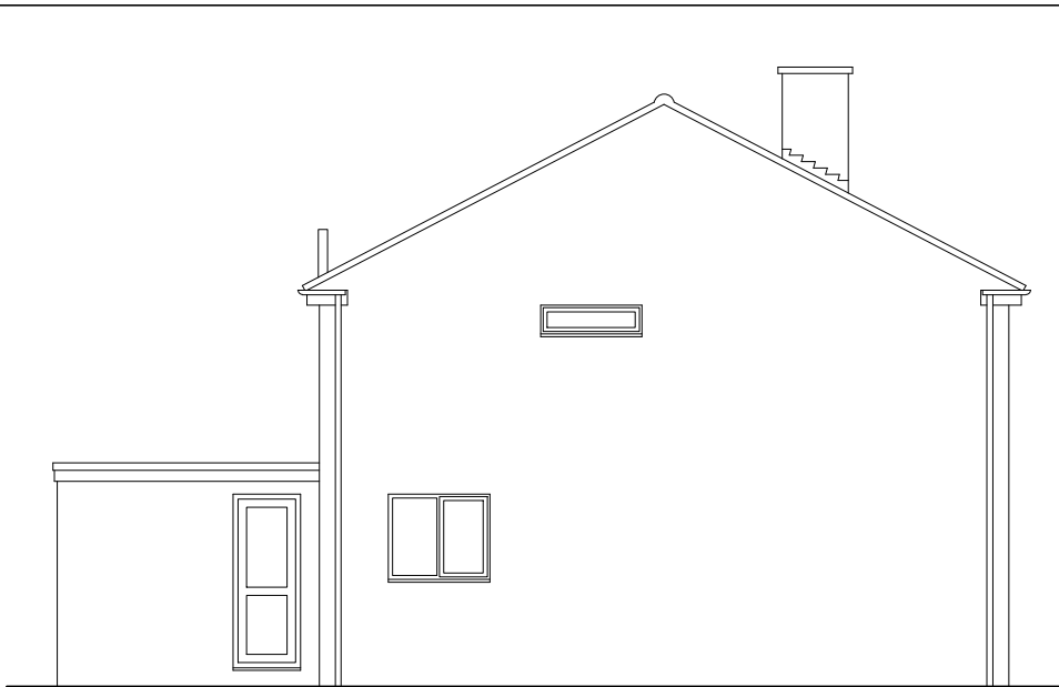
Existing South Elevation (side) 1:100 @ A3
