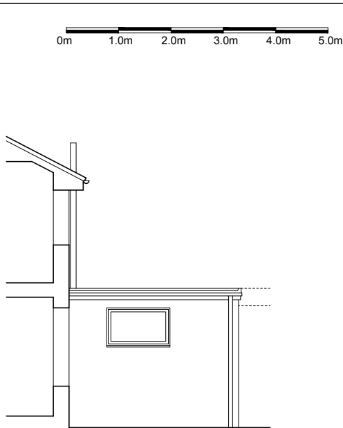
Ex. North Elevation (side) 1:100 @ A3
