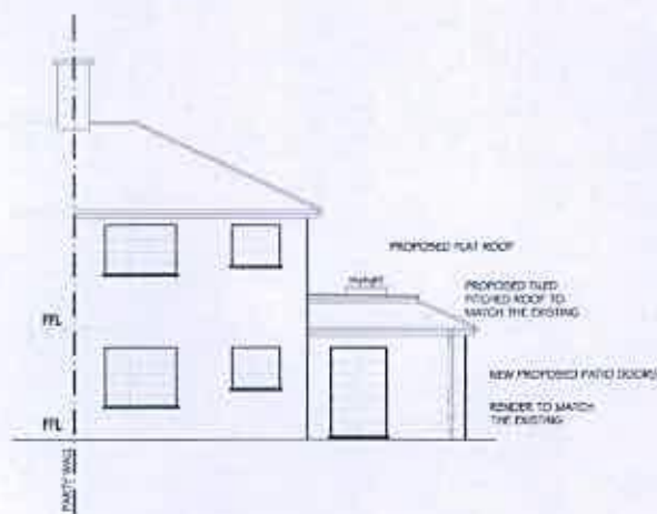
REAR ELEVATION
