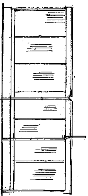
EXISTING SOUTH ELEVATION 1:100
