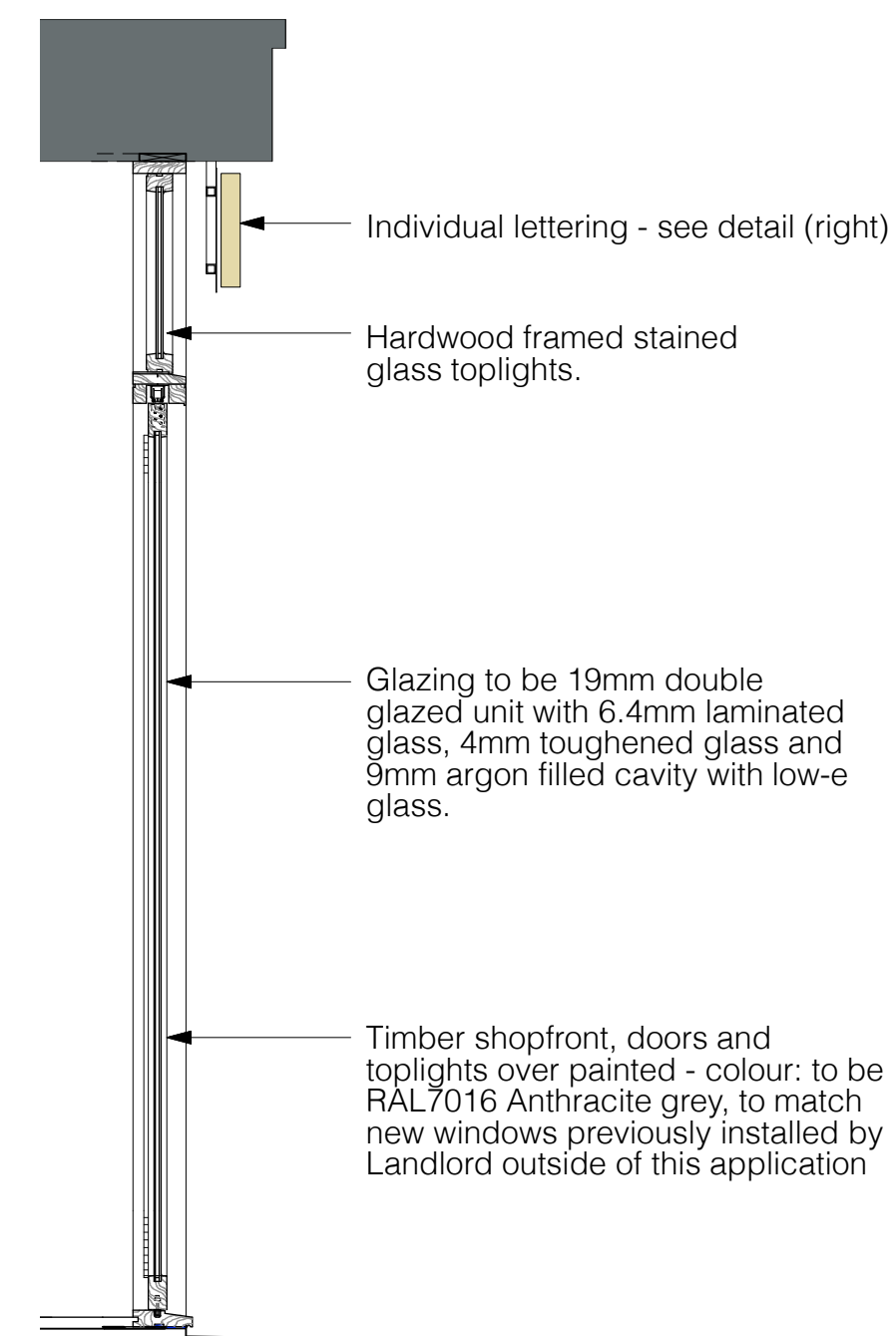
SHOPFRONT SECTION Scale 1:20@A1
