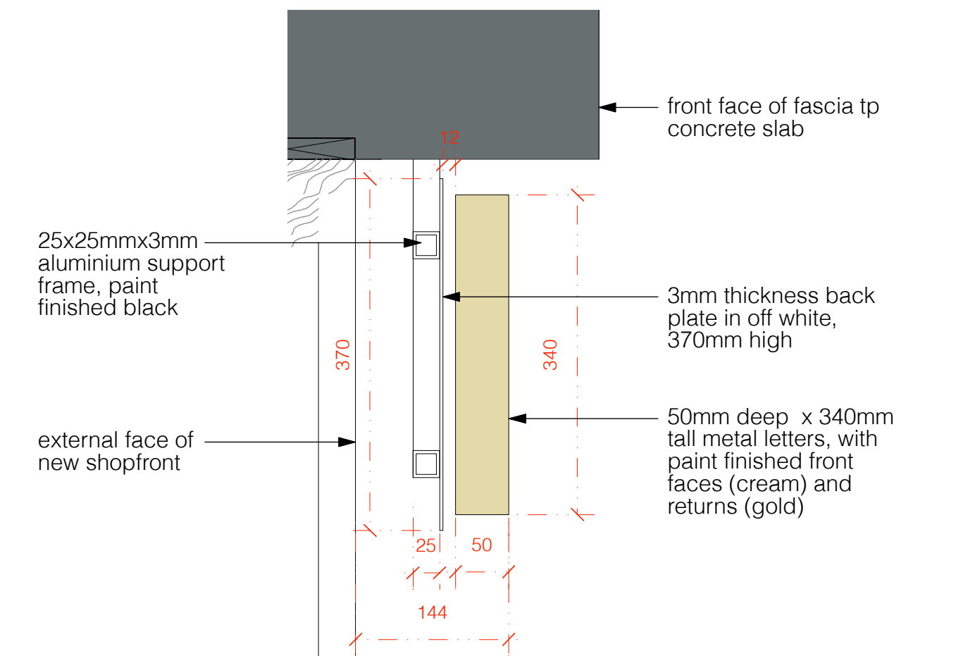
DETAIL SECTION - Scale 1:5@A1
