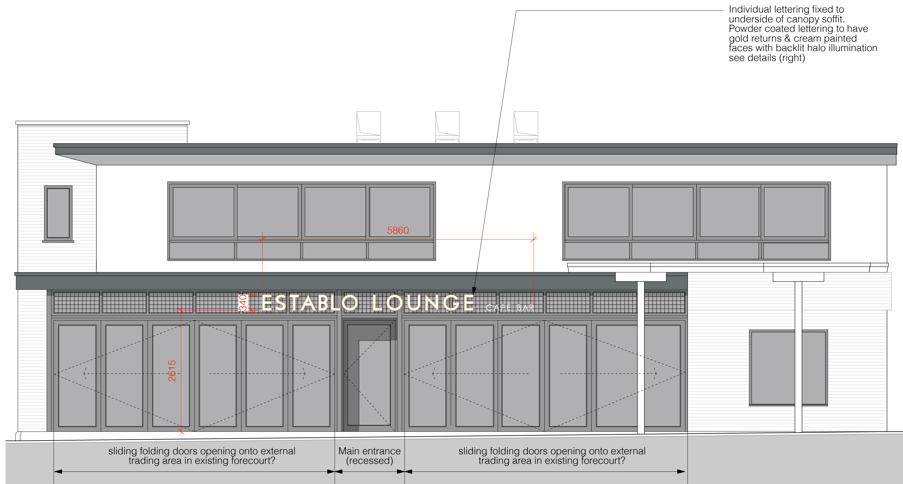
EAST (FRONT) ELEVATION
