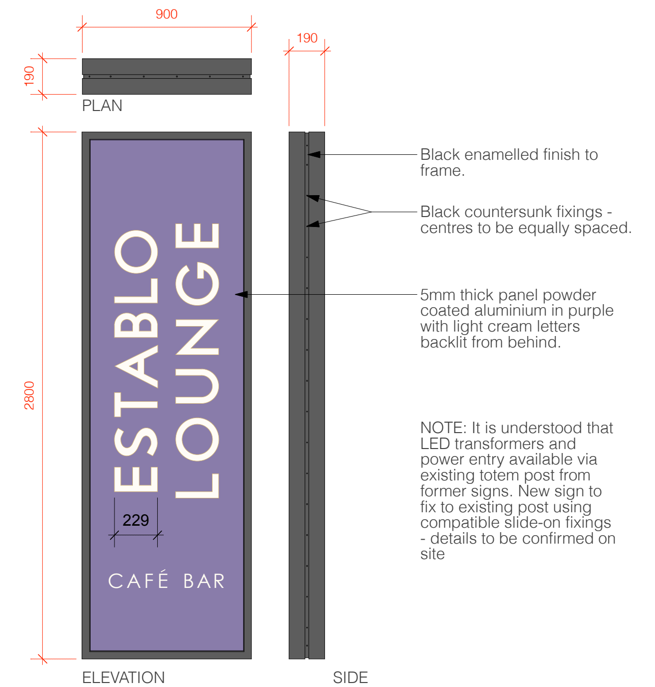
PROPOSED TOTEM SIGN Scale 1:20@A1
