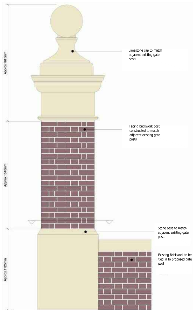
ELEVATION OF PROPOSED PIER (FRONT)
