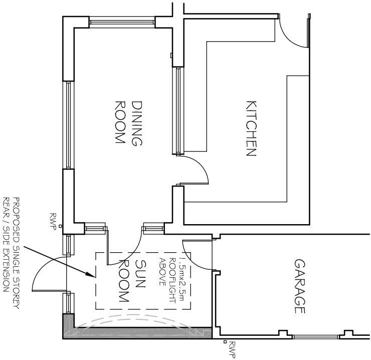
PROPOSED PART FLOOR PLAN
