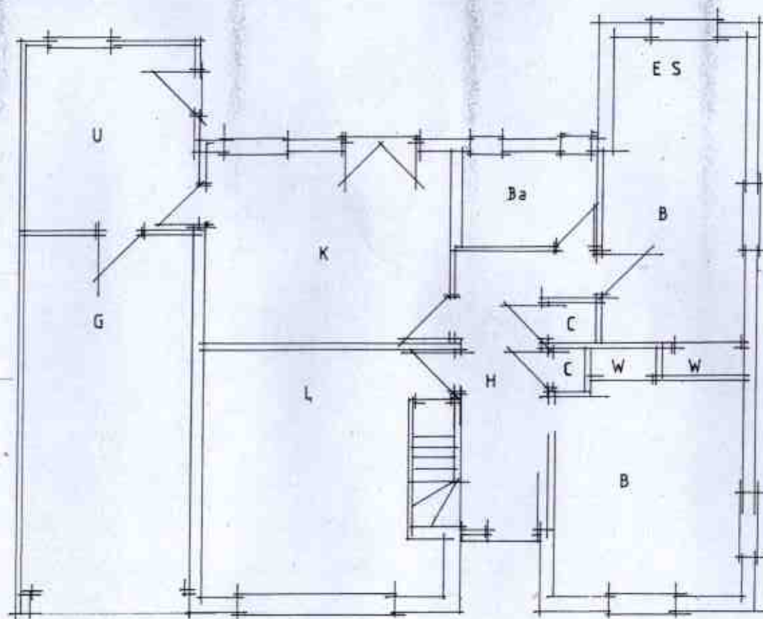
Existing plan 1:100
