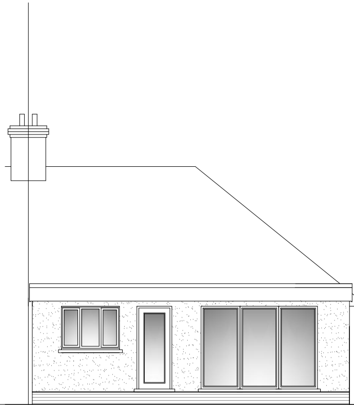
REAR ELEVATION (EAST)
