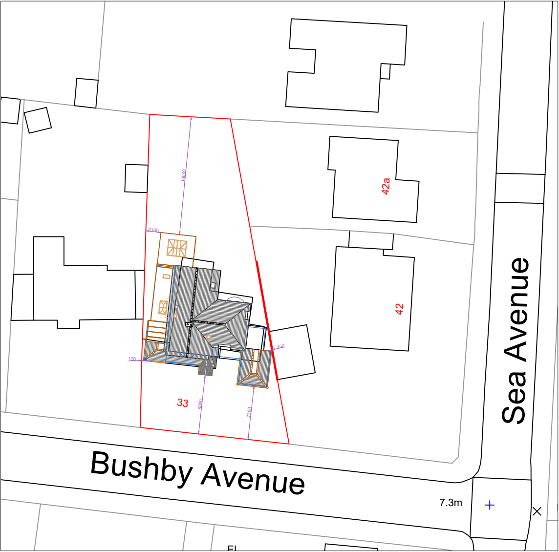
Block Plan
