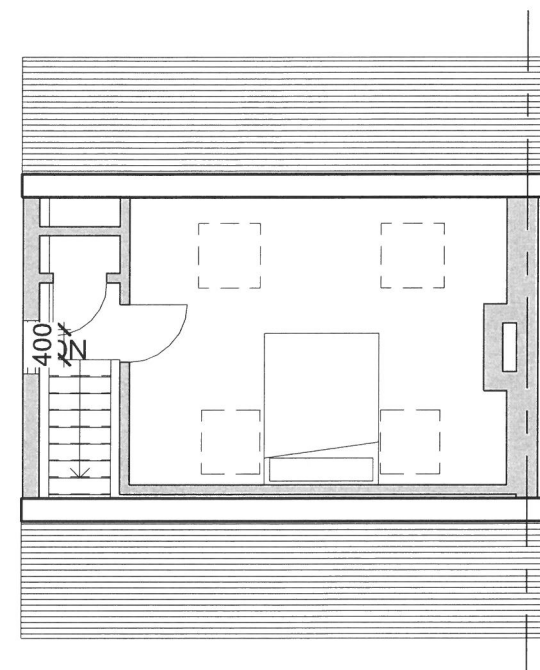
Proposed Loft Plan 1 : 100
