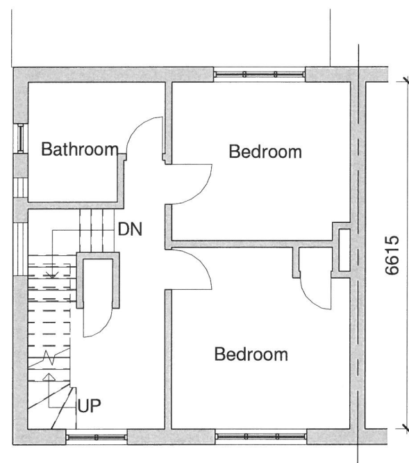
Proposed First Floor 1 : 100
