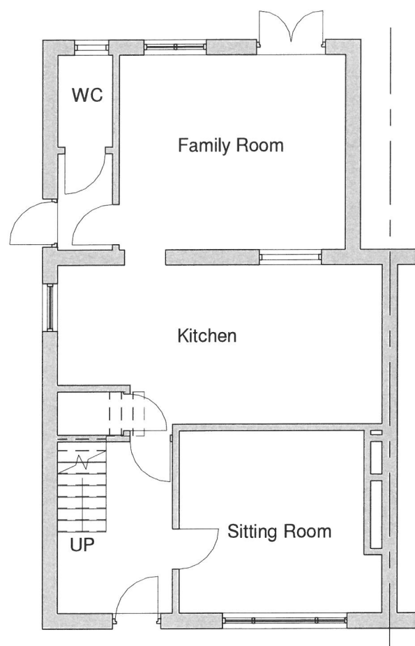
Proposed Ground Floor 1 : 100
