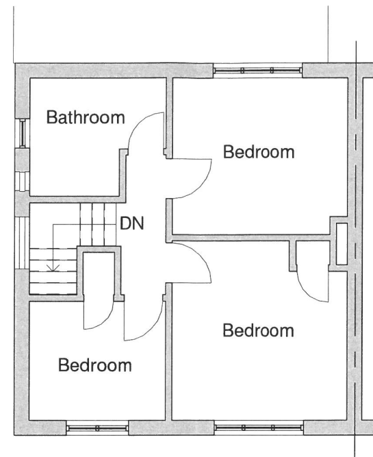
Existing First Floor 1 : 100
