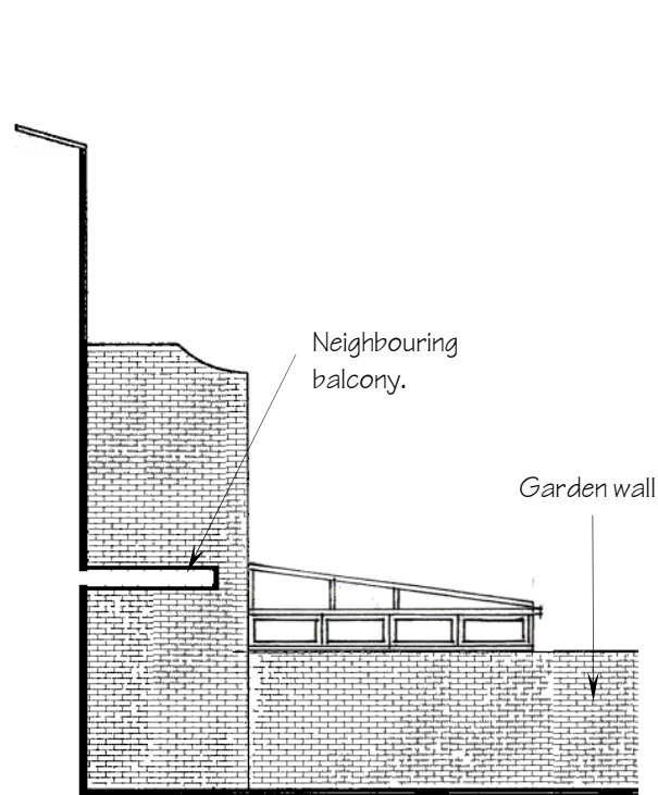
SIDE ELEVATION (WEST)
