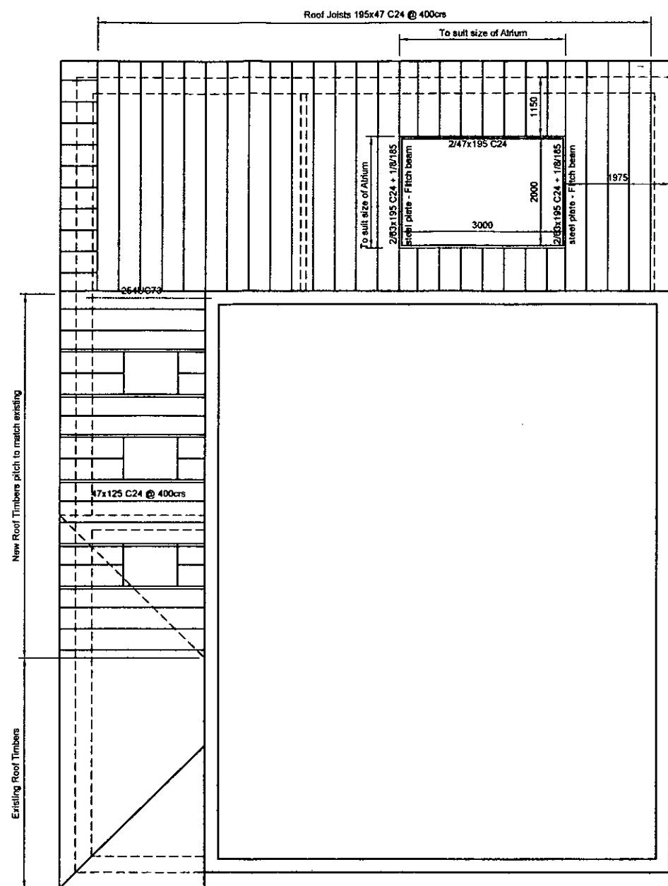
STRUCTURAL ROOF PLAN
