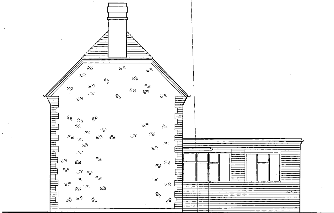
West Side Elevation - as existing The Coach House, 81 The Street, Rustington
