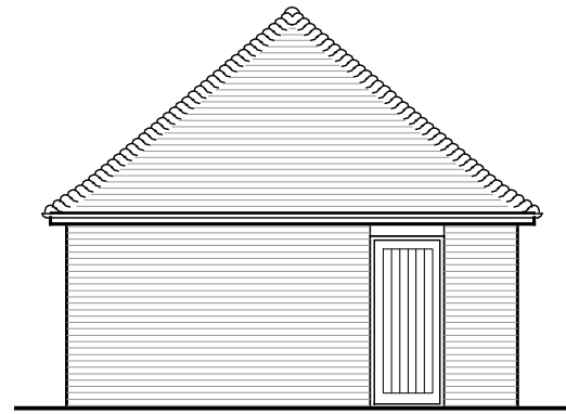
East Elevation
