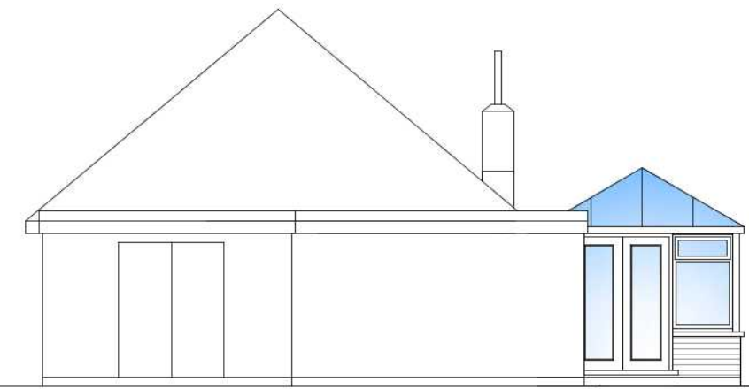
REAR ELEVATION (NORTH)
