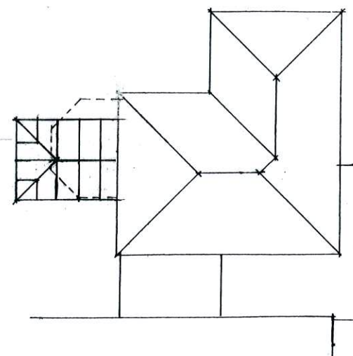
Proposed Roof Plan Scale: 1/200
