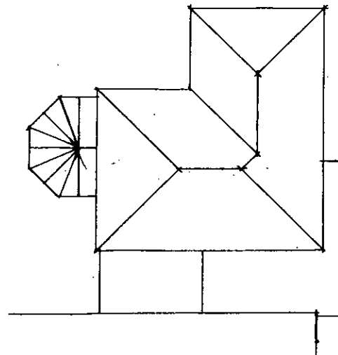
Existing Roof Plan Scale: 1/200
