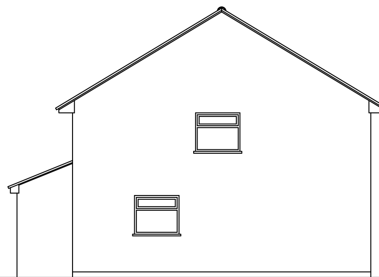
Proposed South Elevation
