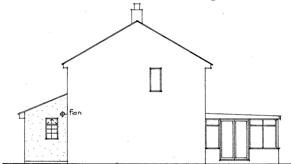
S Elevation
