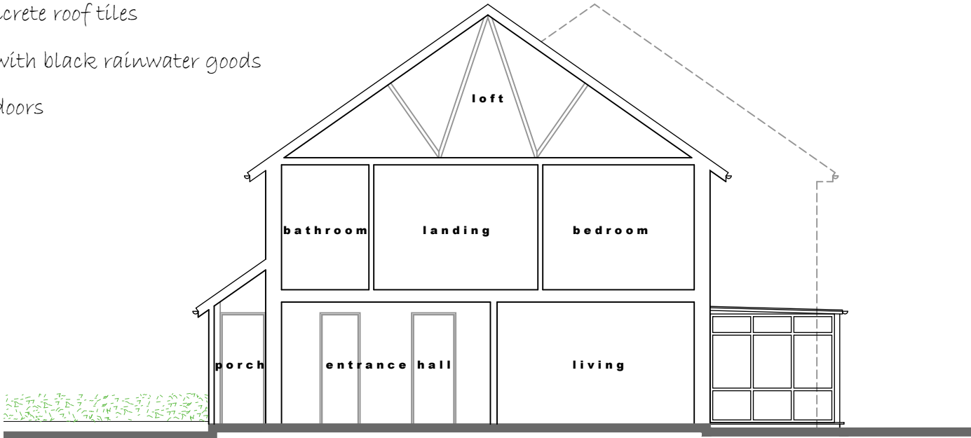
part section / elevation north
