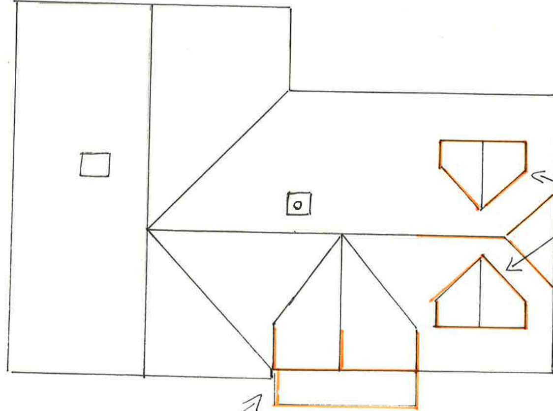
Proposed Roof Plan 1:100 on A3
