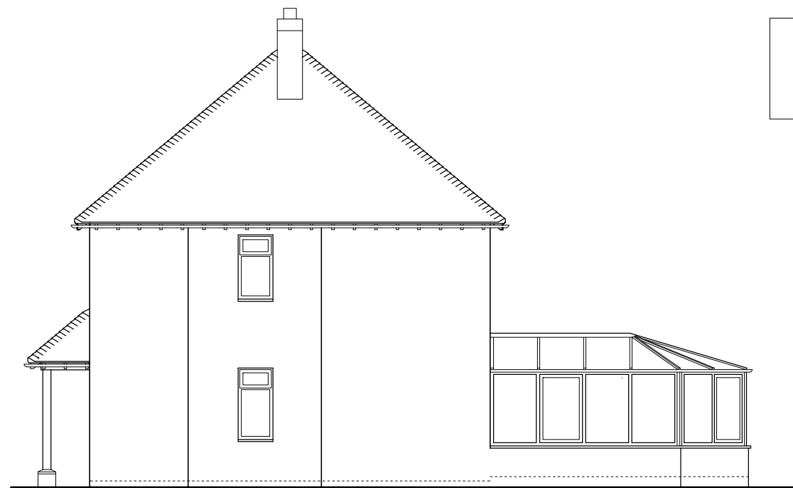
South Elevation
