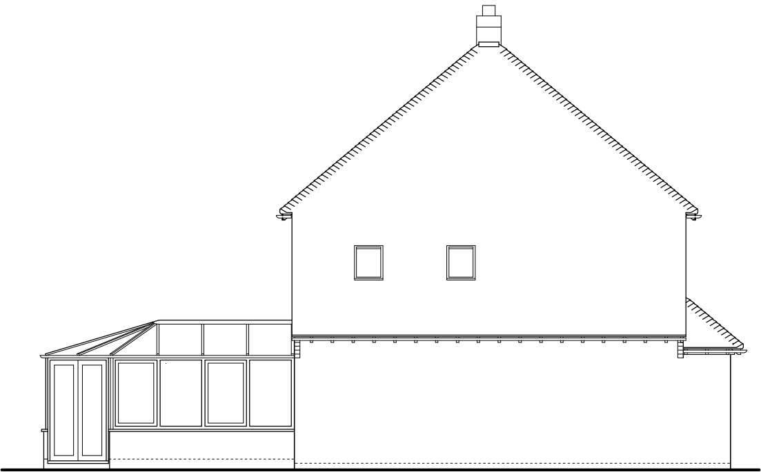
North Elevation
