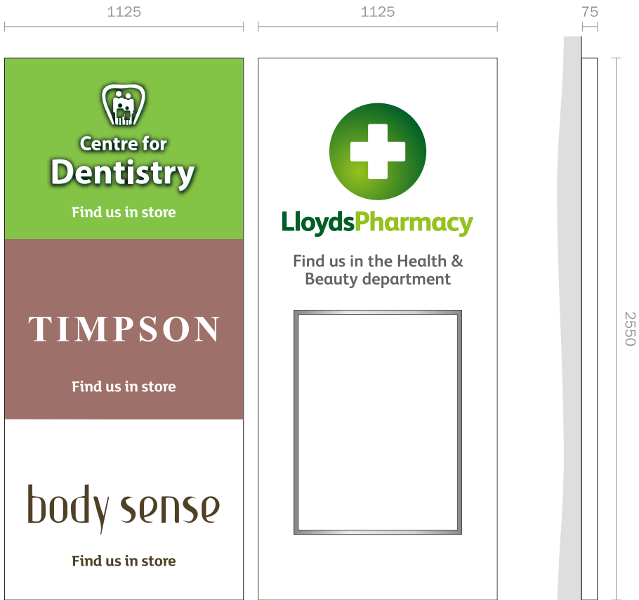
Signs 'G & H' Scale 1:25
