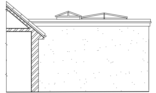
Side Elevation (South-East Facing) (Scale 1:100)
