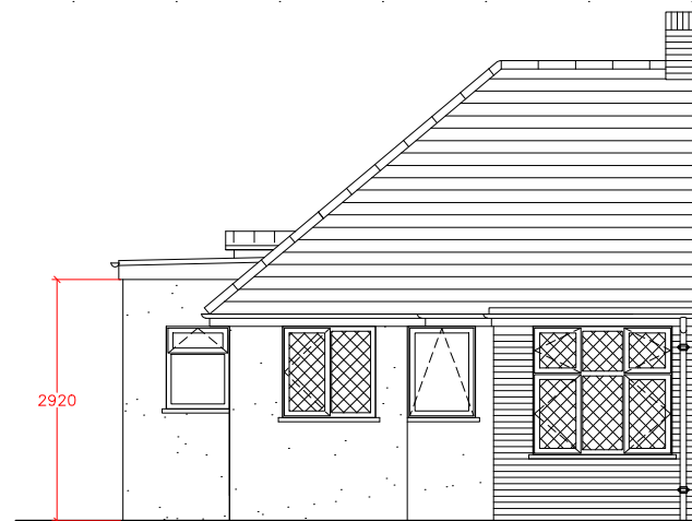
Front Elevation (South-West Facing) (Scale 1:100)
