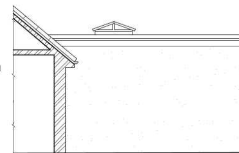
Side Elevation (South-East Facing) (Scale 1:100)
