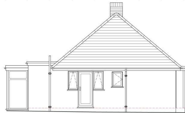
Front Elevation (South-West Facing) (Scale 1:100)
