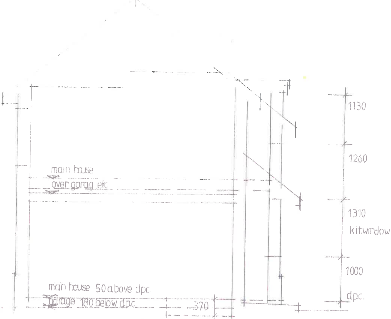
GENERAL CROSS SECTION 1/50
