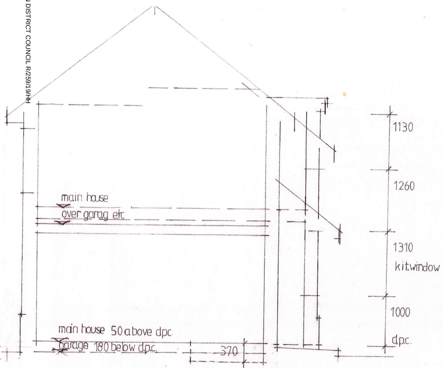
GENERAL CROSS SECTION 1/50
