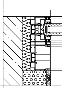
Jambo Detail
