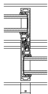
Sill Detail
