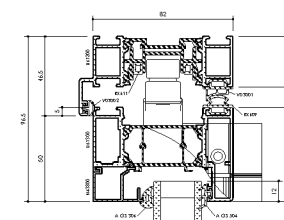
F82 Head
