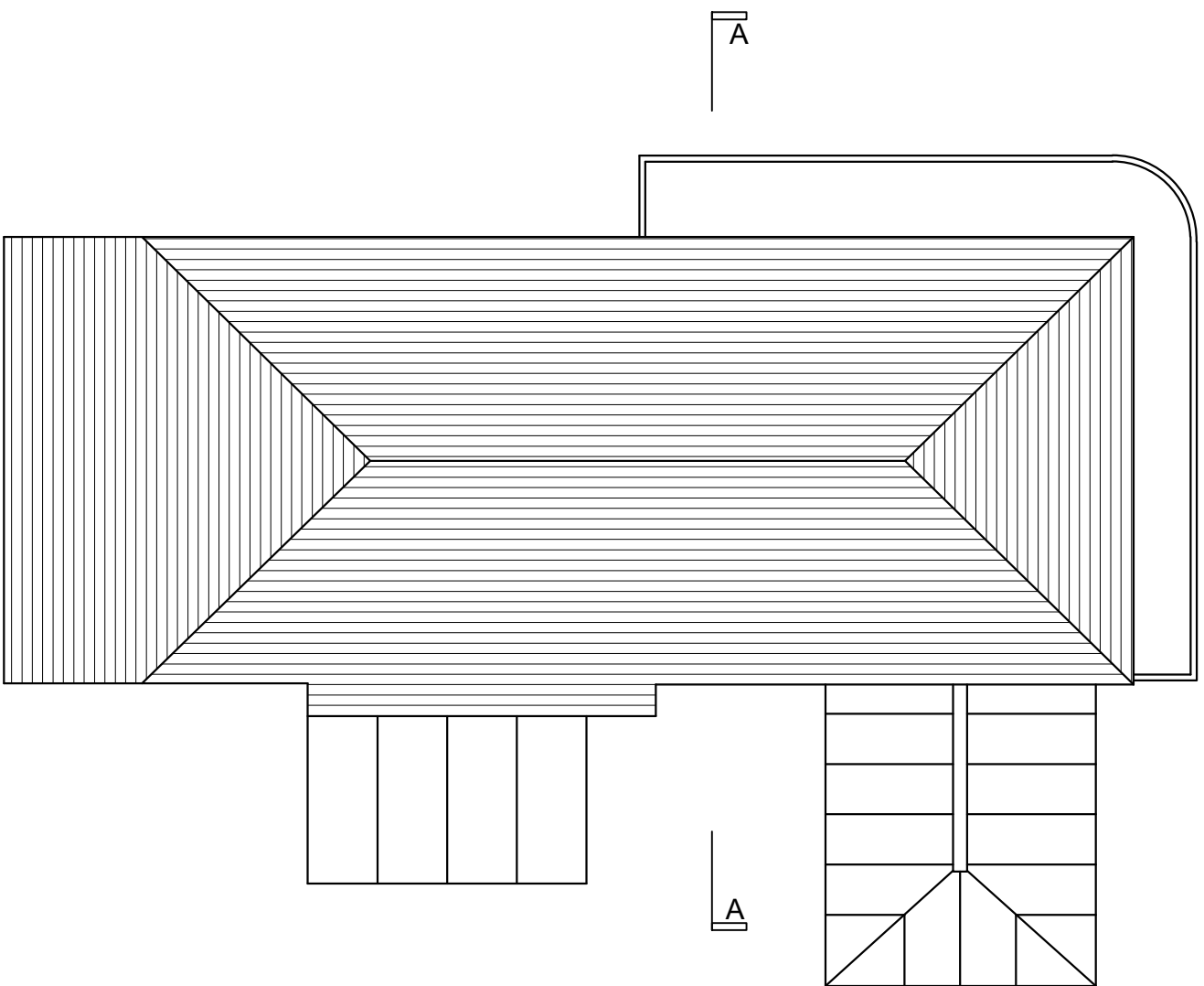
Roof Plan 1:100
