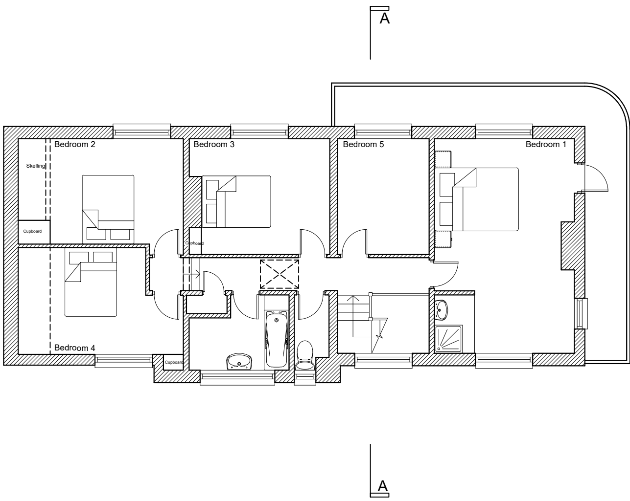
First Floor 1:100
