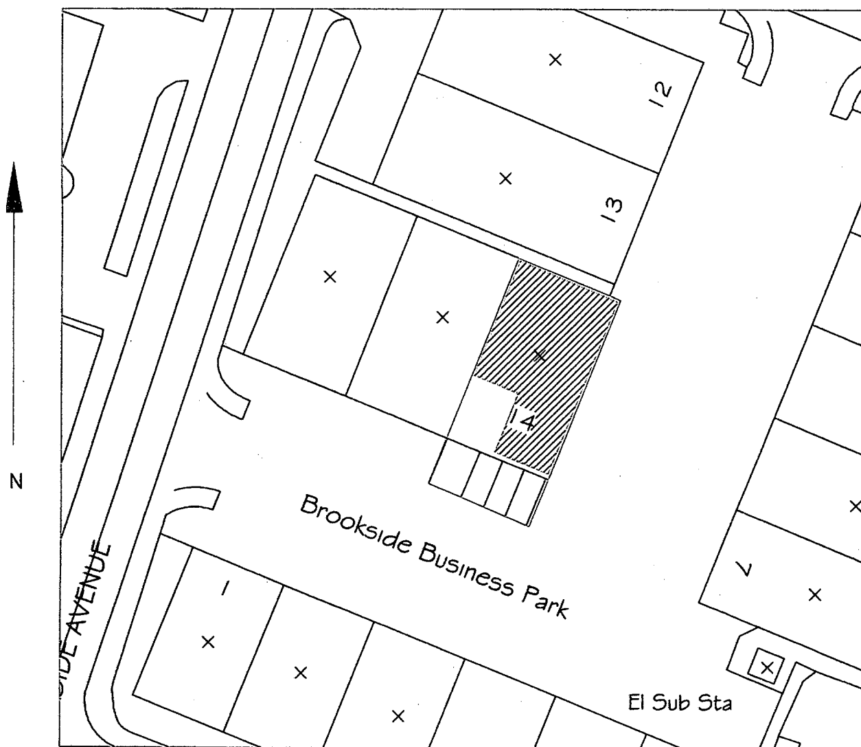
Block Plan @ 1:500 (Hatched area denotes proposed mezzanine)
