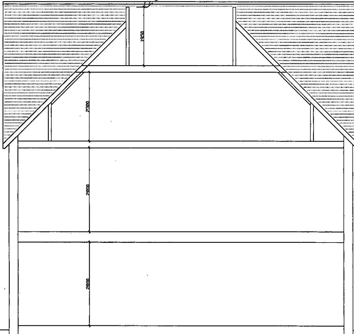
Proposed Typical Section, Scale 1:50
