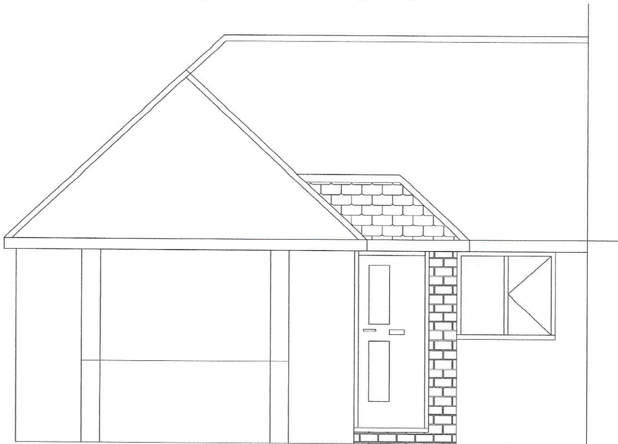
Existing Front Elevation (West)
