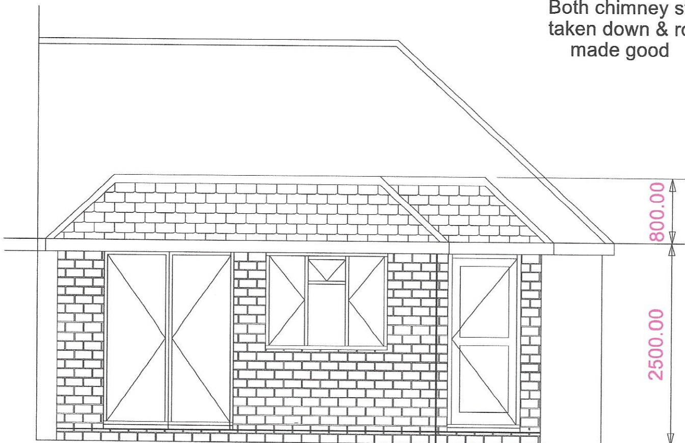
Existing Rear Elevation without sunroom
