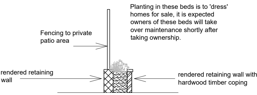
Section B-B 1:50
