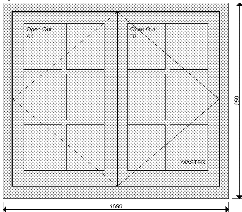
Flush casement window, Opening out, Viewed internally
