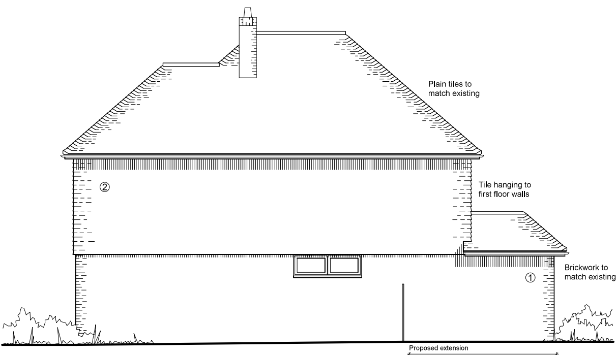
South Elevation
