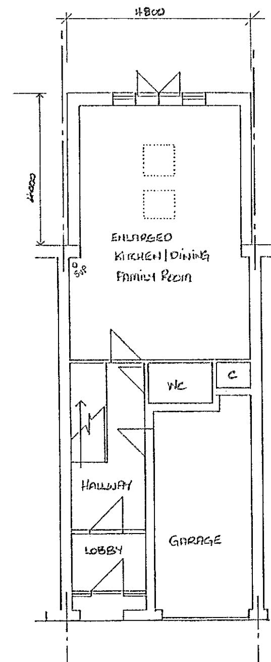
PROPOSED GROUND FLOOR
